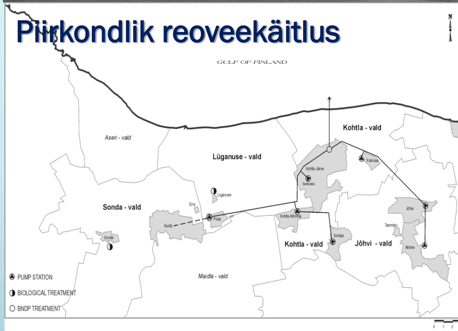
Proposed Wastewater Management System
